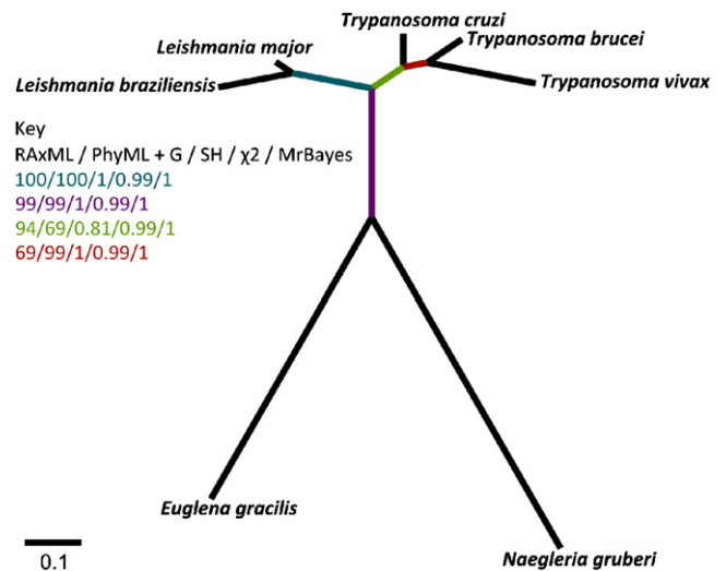
Fig. 4. Bayesian analysis (MrBayes) including data from three additional taxa, L. braziliensis , T. vivax and E. gracilis . Topology support values in the key match corresponding internal branches of the tree. The green branch defines monophyly of Trypanosoma to the exclusion of both the Leishmania species.
